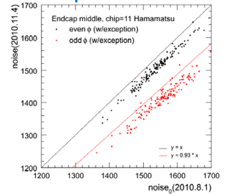
chip 11
