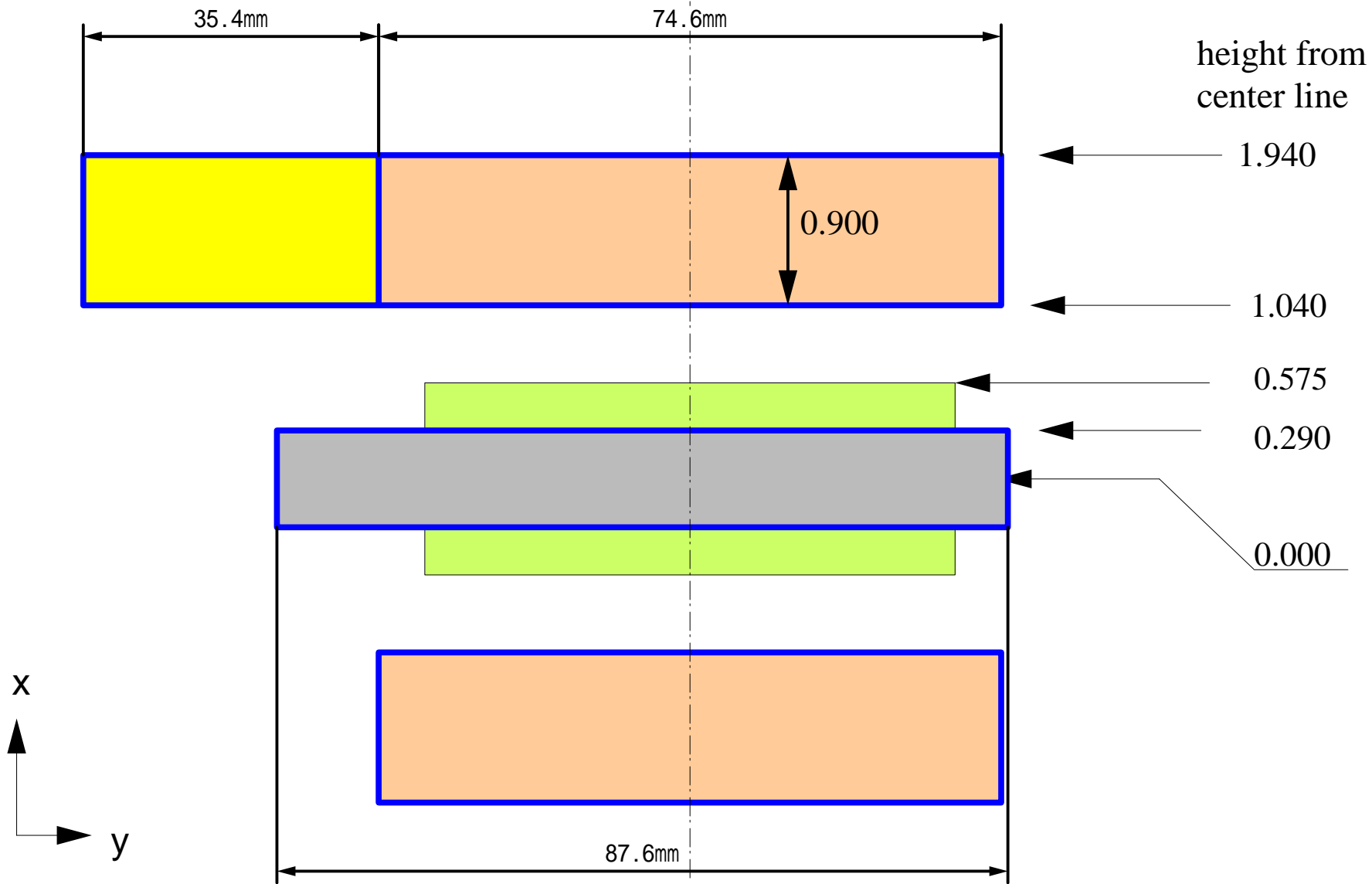
BARREL SENSOR MODULE: CROSS SECTION B-B'
