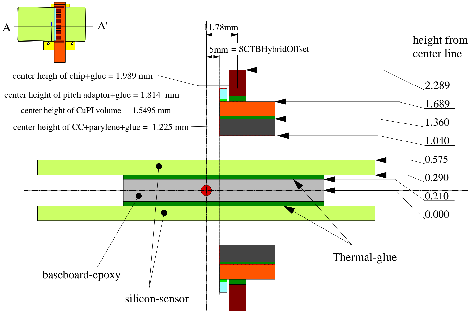
BARREL SENSOR MODULE: CROSS SECTION A-A' ref. SCT-BM-FCR-4 Table-1, TB-0059-601-01
