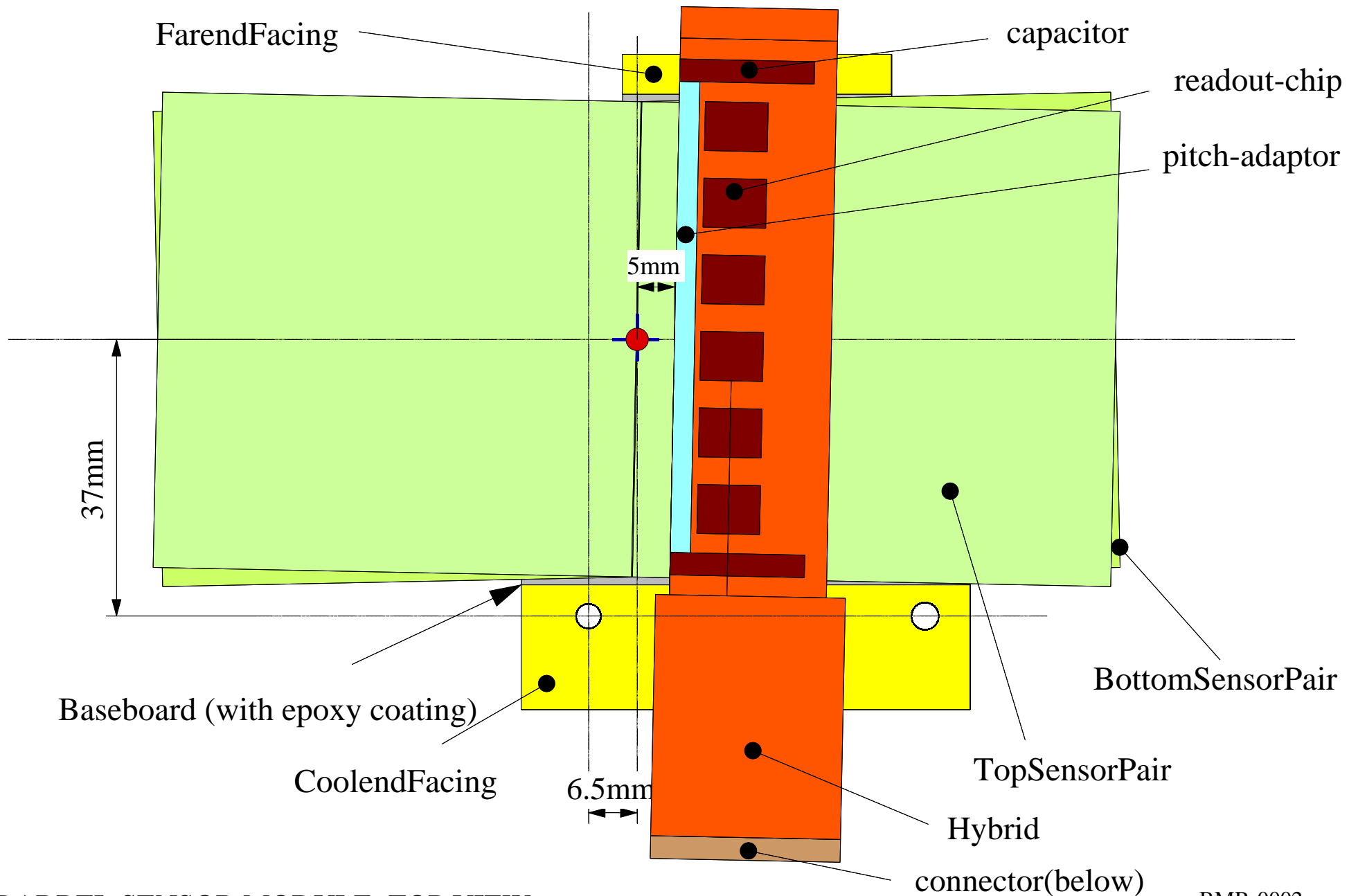
BARREL SENSOR MODULE: TOP VIEW
