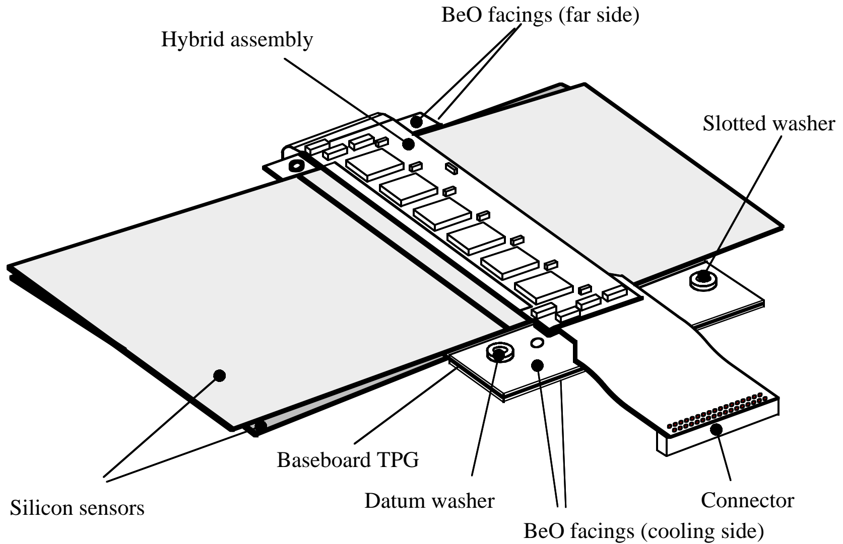
BARREL SENSOR MODULE: BIRDEYE VIEW
