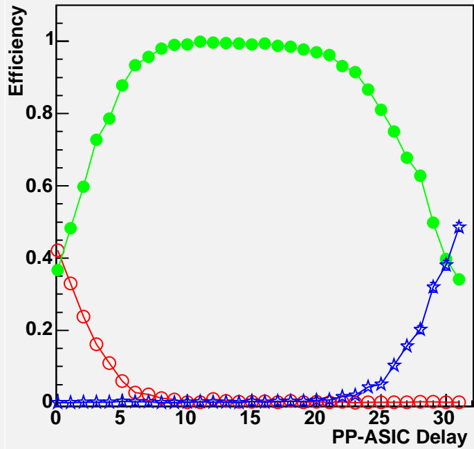
Triplet Wire Coincidence Efficiency
