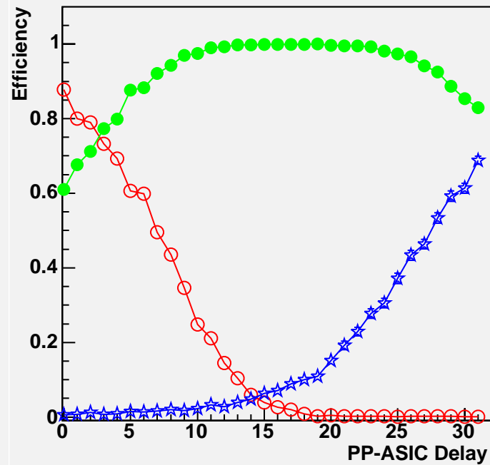
Triplet Strip Coincidence Efficiency
