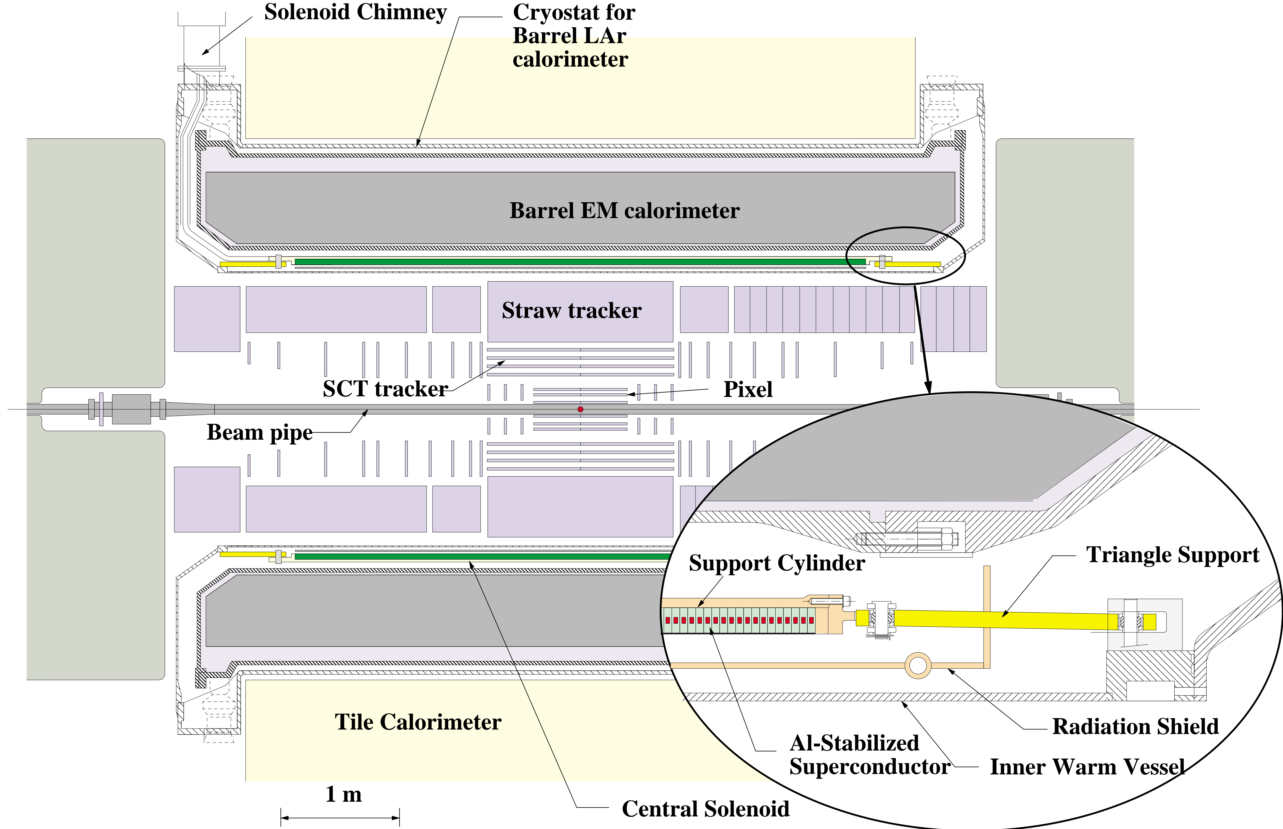
ATLAS Central Solenoid
